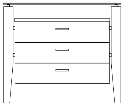
MEUBLE D'APPOINT / SIDE BOARD 15 x 38 x H 32 MIKA MAP 1538
